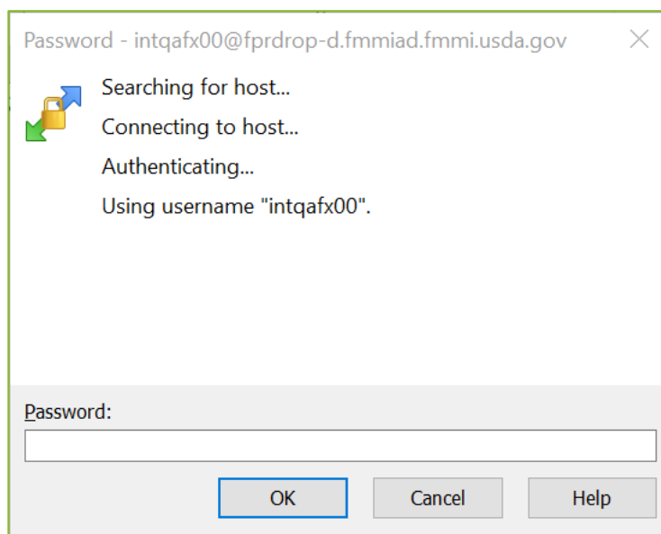
Figure 8: WinSCP Login
